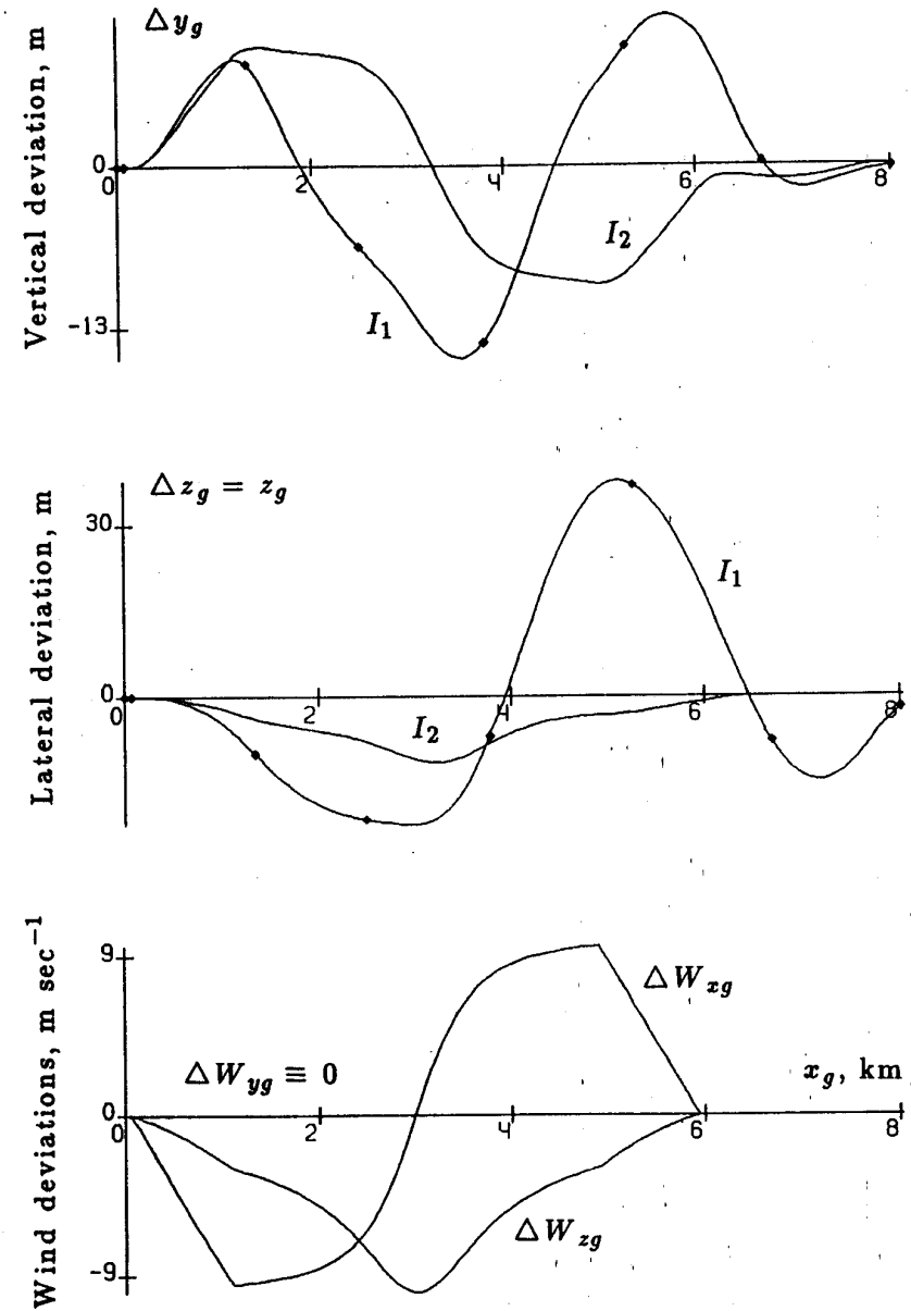
Fig. 6b. Landing simulation results for Model M3; downburst center DX = 3000 m, DZ = 600 m.
