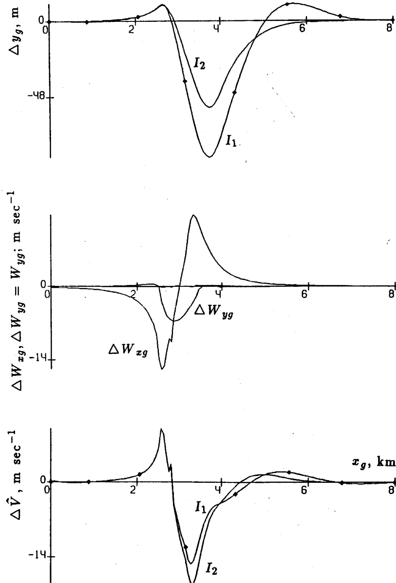
Fig. 7a. Deviation histories: altitude y_g , wind velocity components W_{xg} and W_{yg} , relative velocity \hat{V} ; Model M2, downburst center DX = 3000 m, DZ = 200 m.
