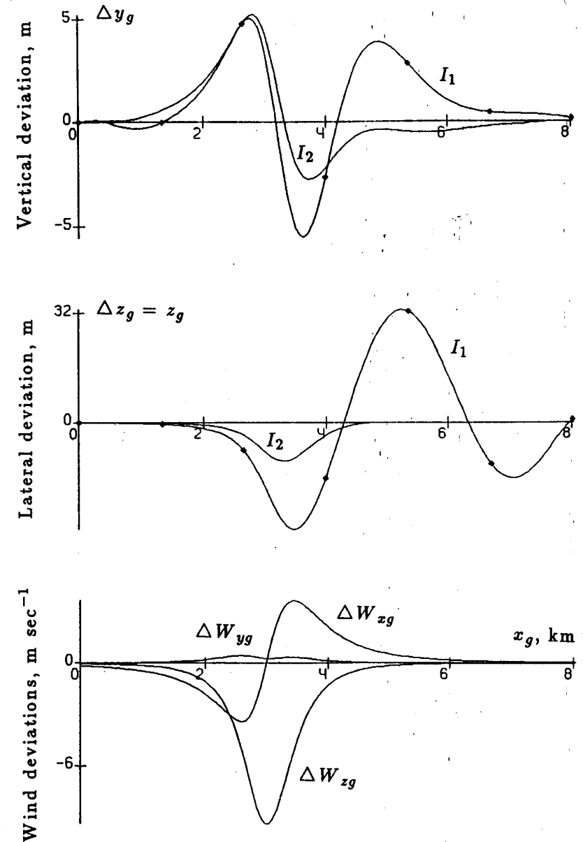
Fig. 5b. Landing simulation results for Model M2; downburst center DX = 3000 m, DZ = 600 m.
