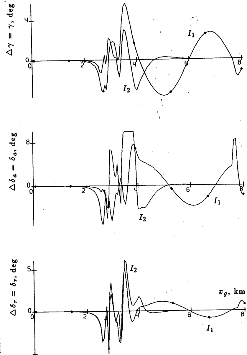
Fig. 7d. Deviation histories: bank angle \gamma , aileron deflection \delta_a , rudder deflection \delta_r ; Model M2, downburst center DX = 3000 m, DZ = 200 m.
