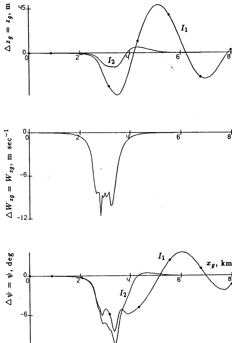
Fig. 7c. Deviation histories: lateral position z_g , wind velocity component W_{zg} , yaw angle \psi ; Model M2, downburst center DX = 3000 m, DZ = 200 m.
