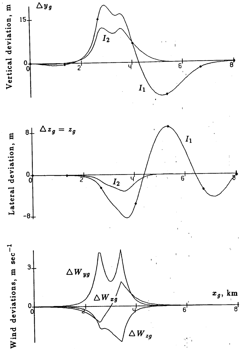
Fig. 4b. Landing simulation results for Model M1; downburst center DX = 3000 m, DZ = 600 m.
