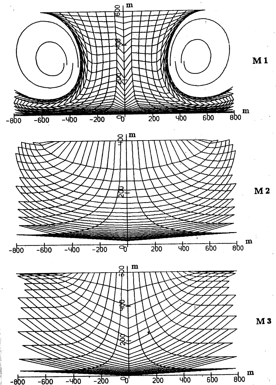
Fig. 3. Downburst models; wind velocity structure in a vertical plane.
