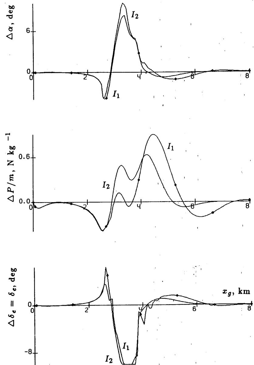
Fig. 7b. Deviation histories: angle attack \alpha , ratio P/m , elevator deflection \delta_e ; Model M2, downburst center DX = 3000 m, DZ = 200 m.
