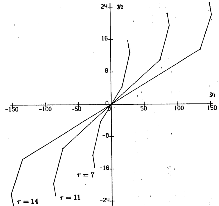
Fig. 2. Switch lines.
