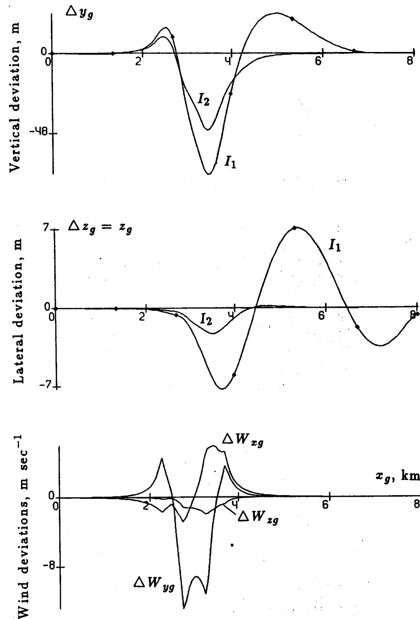
Fig. 4a. Landing simulation results for Model M1; downburst center DX = 3000 m, DZ = 100 m.
