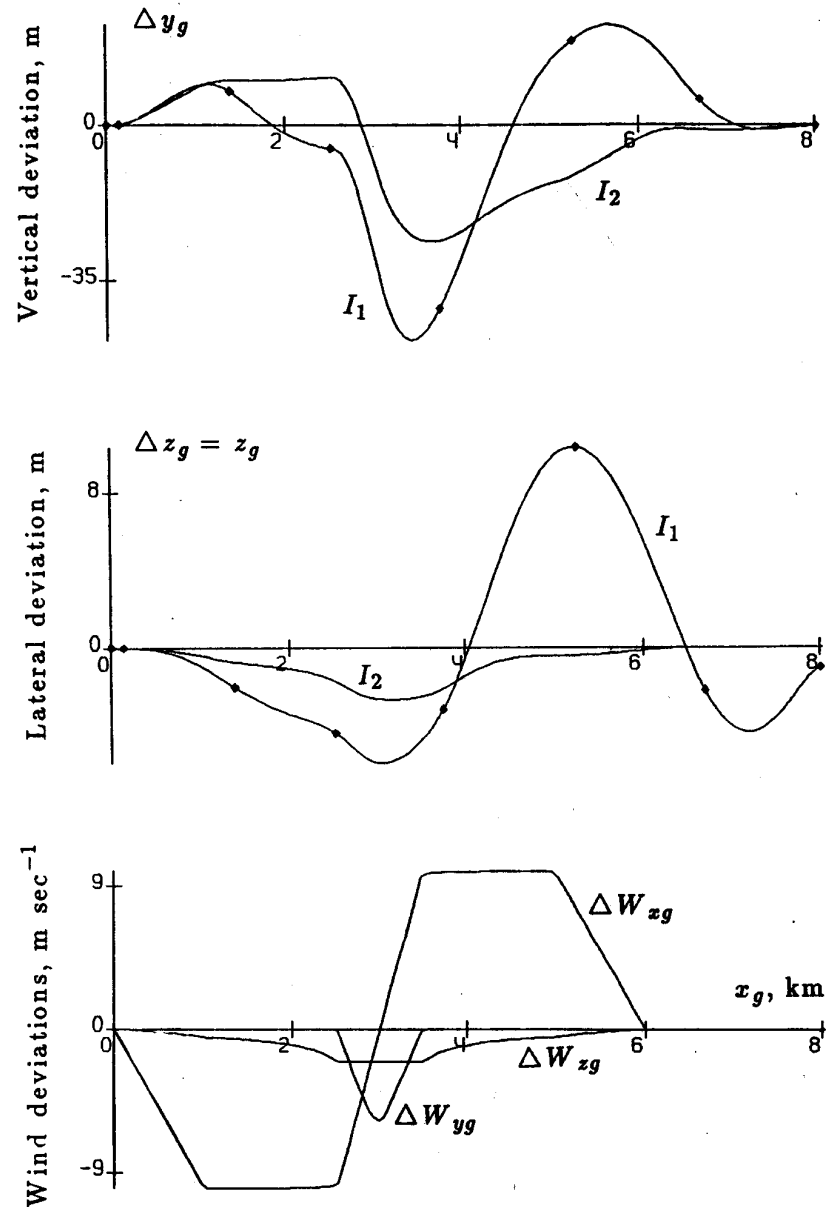
Fig. 6a. Landing simulation results for Model M3; downburst center DX = 3000 m, DZ = 100 m.
