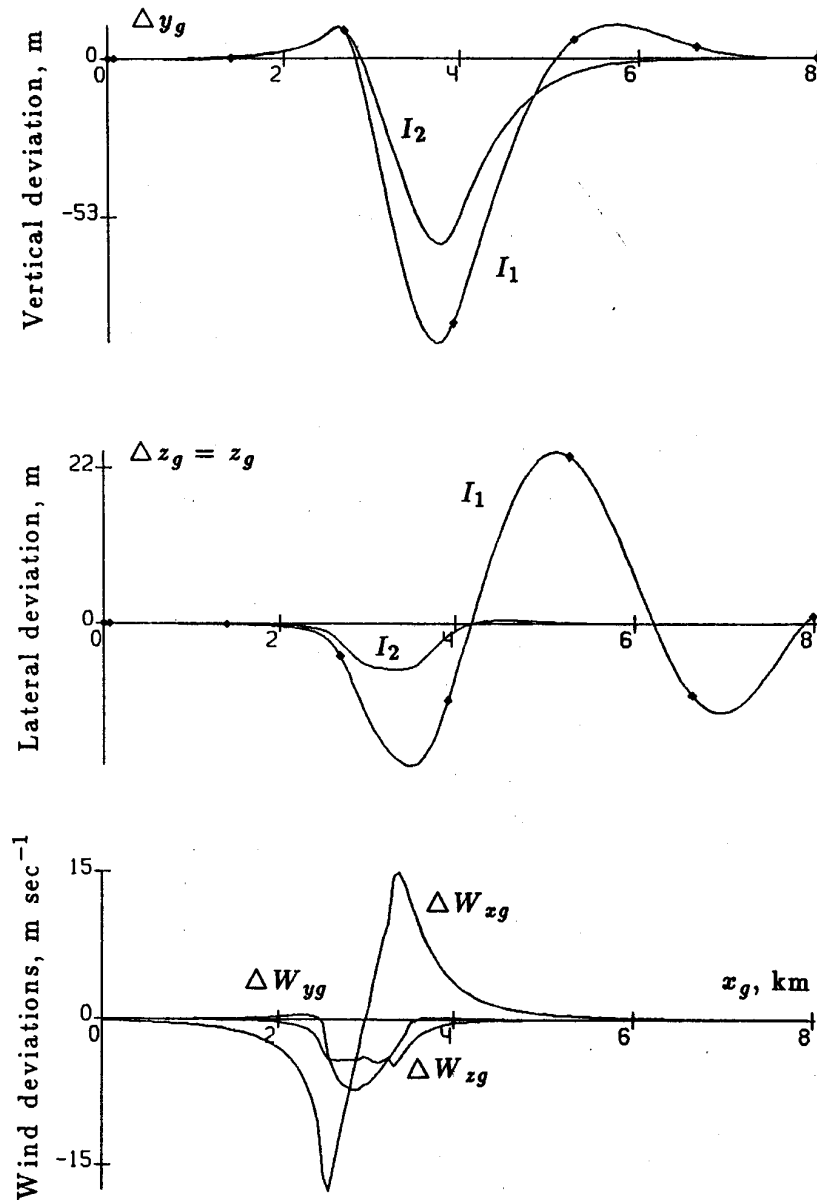
Fig. 5a. Landing simulation results for Model M2; downburst center DX = 3000 m, DZ = 100 m.
