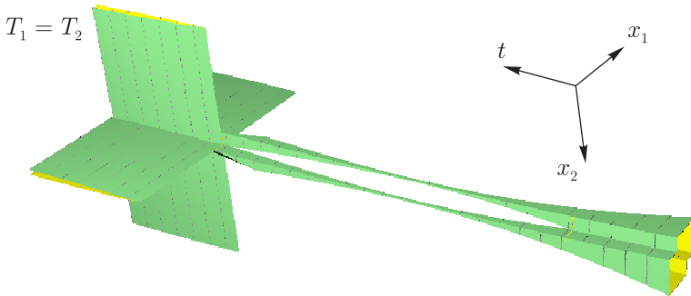
Figure13. Example 5. Narrow throats in a problem with three objects having dynamics (15)
