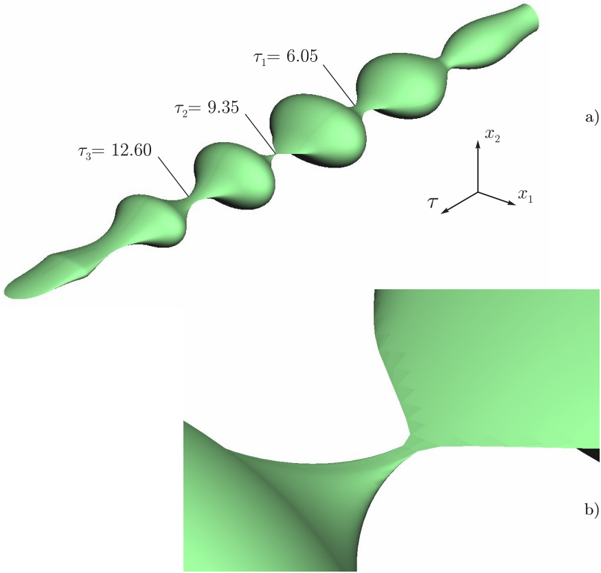
Figure12. Example 4. a) A general view of a level set with three narrow throats, c = 0.397 ; b) An enlarged view of the narrowest of the throats (the middle one)
