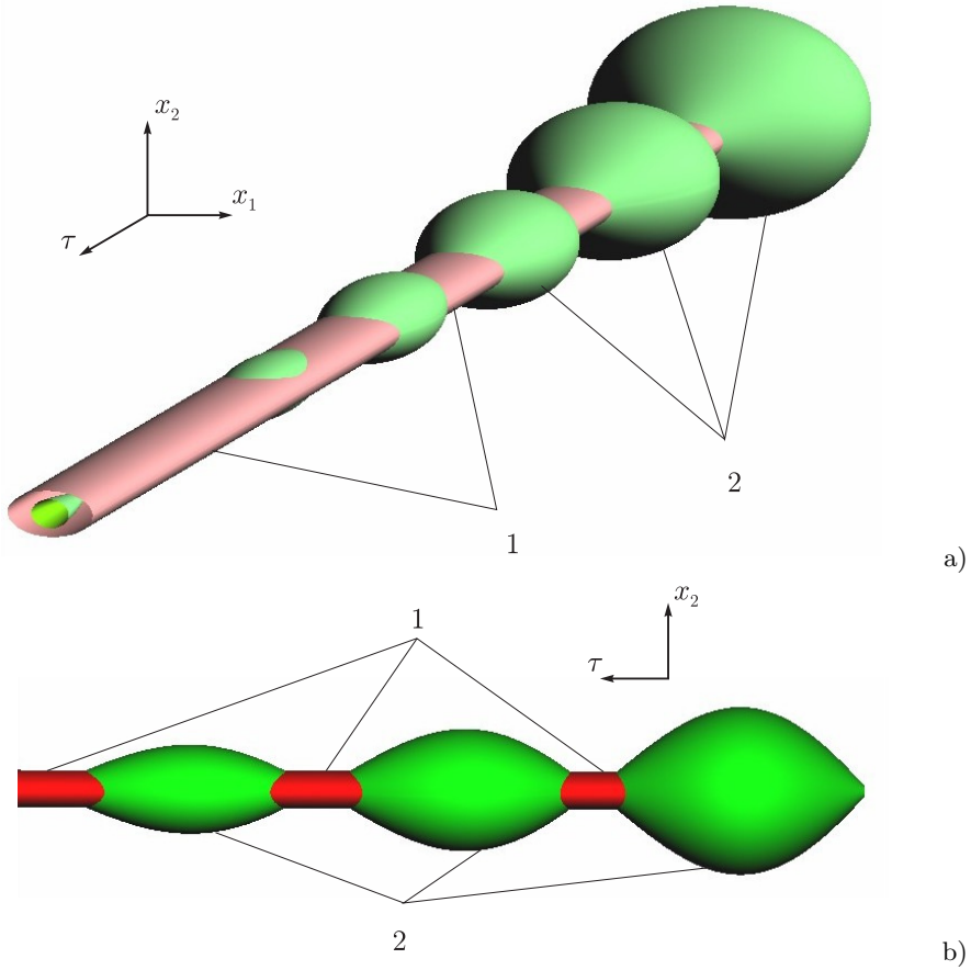
Figure 4. Example 2. Two views of the vectogram tubes. Number 1 denotes the tube of the first player (the set \mathcal{P} ), number 2 corresponds to the second player's vectogram tube (the set \mathcal{Q} )
