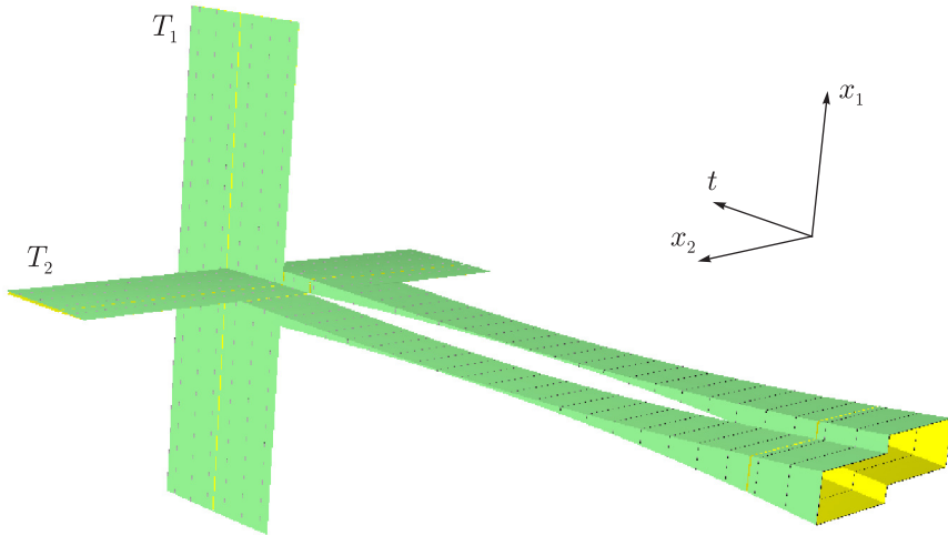
Figure15. Example 7. The level set W_{0.525} for the pursuers' dynamics of type (18); the pursuers have different parameters of the dynamics
