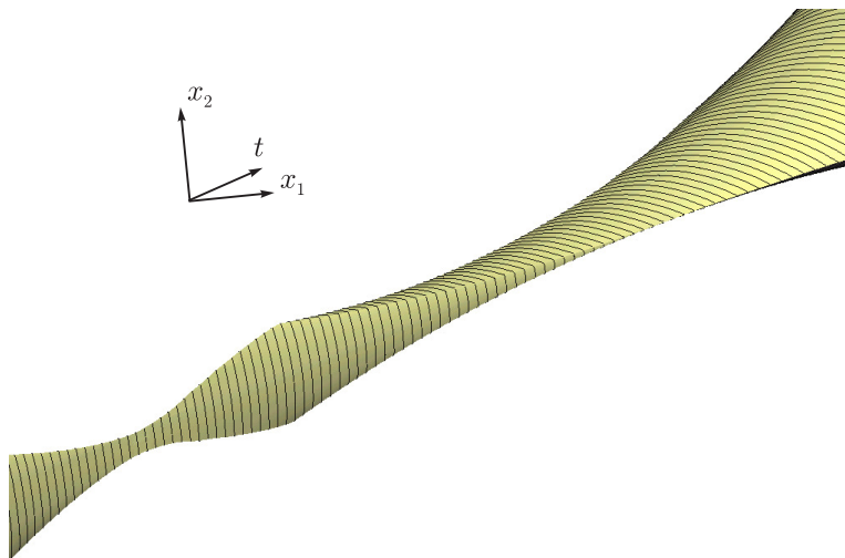
Figure3. A large view of the narrow throat
