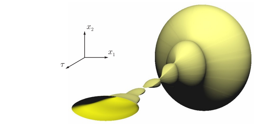
Figure6. Example 2. A general view of the level set with a narrow throat, c = 2.45100
