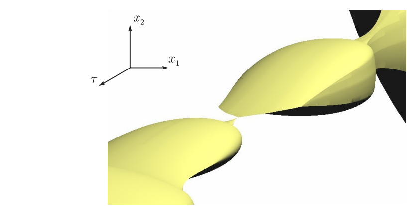
Figure7. A large view of the narrow throat
