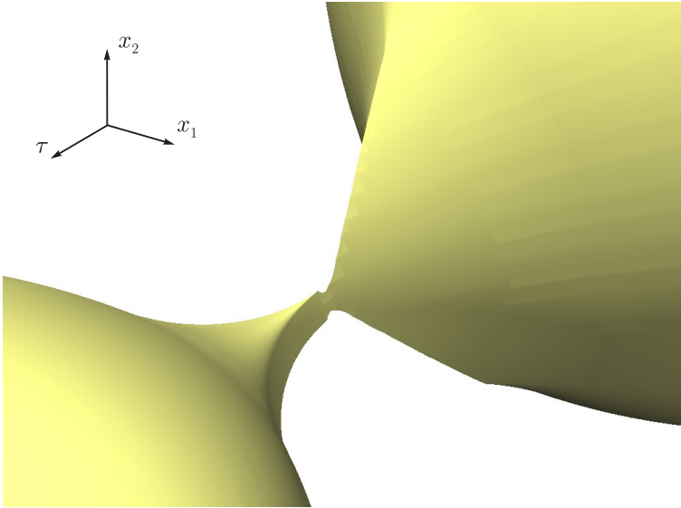
Figure10. An enlarged view of the first (in the backward time) narrow throat
