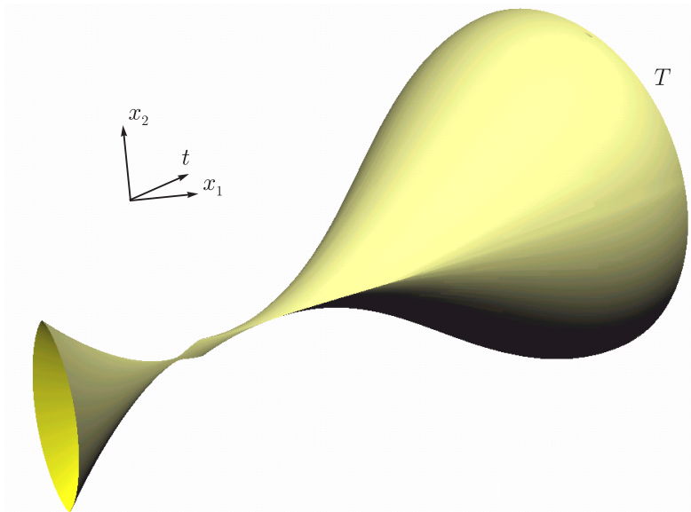
Figure2. Example 1. A general view of the level set of the value function with a narrow throat
