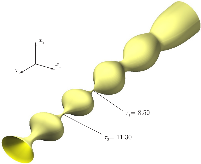
Figure9. Example 3. A general view of the level set with two narrow throats, c = 1.2
