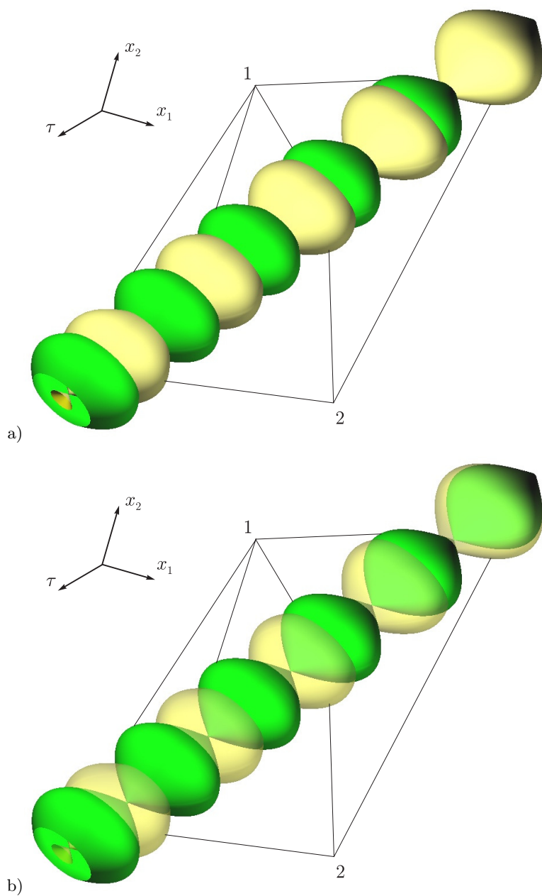
Figure8. Example 3. A general view of the vectogram tubes. Number 1 denotes the tube of the first player (the set \mathcal{P} ), number 2 corresponds to the second player's vectogram tube (the set \mathcal{Q} ). In subfigure b), the tube of the second player is transparent
