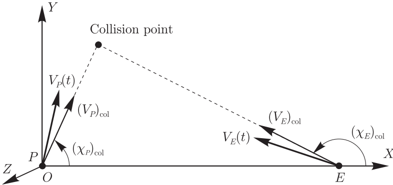
Figure1. The geometry of the three-dimensional interception. The actual realizations of the velocity vectors V_P(t) and V_E(t) are close to the nominal values (V_P)_{col} and (V_E)_{col}
