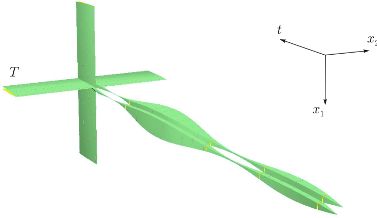
Figure14. Example 6. A level set for example 2 with two narrow throats
