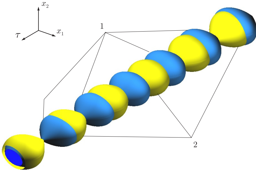
Figure 11. Example 4. A large view of the vectogram tubes. Number 1 denotes the tube of the first player (the set \mathcal{P} ), number 2 corresponds to the second player's vectogram tube (the set \mathcal{Q} )
