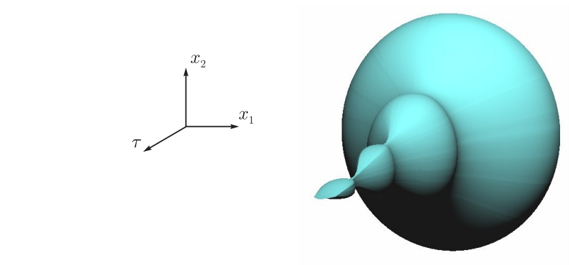
Figure5. Example 2. A broken level set close to the critical one, c = 2.45098
